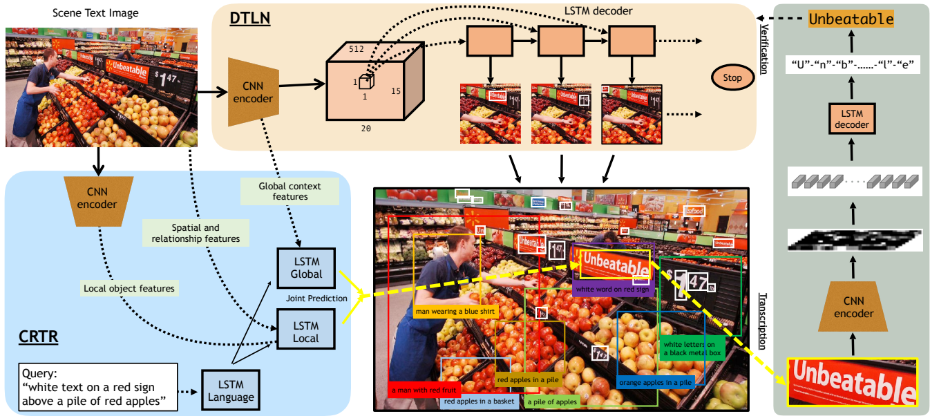
Fig. 2: The architecture of the proposed Dense Text Localization Network (DTLN) and Context Reasoning Text Retrieval (CRTR) Models. For an input image, the DTLN model directly decodes the CNN features into a variable length set of text instance candidates. The CRTR model pools the information from three different LSTM models, and jointly scores and ranks the candidate text regions which are generated by DTLN. The rightmost recurrent text recognition module helps further extend the applicability of DTLN and CRTR models, by transcribing the retrieved text regions to precise literal character codes for verification.
