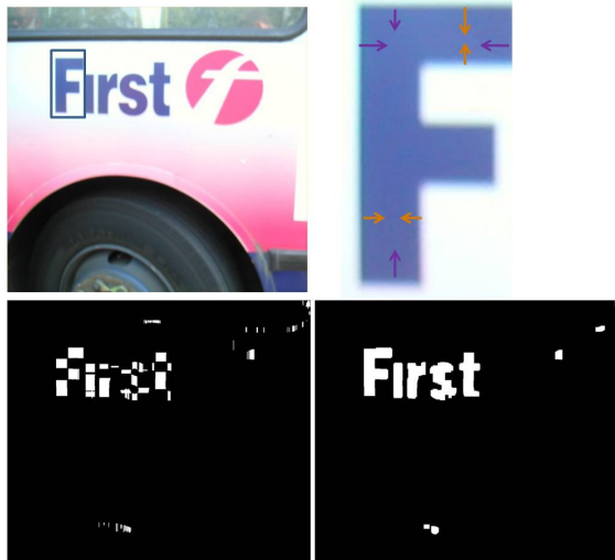
Fig. 5. Connecting path of pixel couple along the larger side of rectangle stroke is analyzed in the second round partition. Top row shows pixel couples in purple across the larger side of rectangle strokes. Bottom row presents the partitioned components obtained from the first round and the second round respectively.
