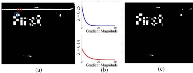
Fig. 4. (a) Two connecting paths of pixel couples marked by blue and red circles respectively. (b) The corresponding exponential distribution of gradient magnitudes on the connecting paths. (c) Partitioned components obtained from the first round.
