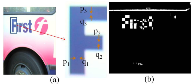
Fig. 3. (a) Examples of pixel couples; (b) connecting paths of all pixel couples are marked as white foreground while other pixels are marked as black background.
