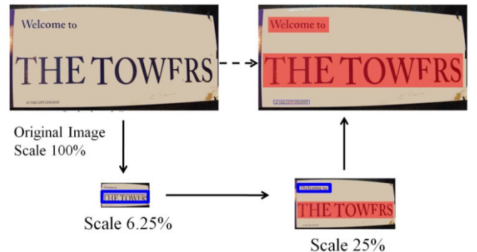
Fig. 11. Multi-scale computing. Regions detected at the current scale level are shown as blue rectangles; red regions containing the characters processed at coarser scale level will be skipped.
