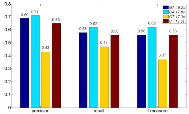
Fig. 12. The performance evaluation of the 4 combinations of partition and grouping on the Robust Reading Dataset, where the box presents the average time of text string detection in each scene image.
