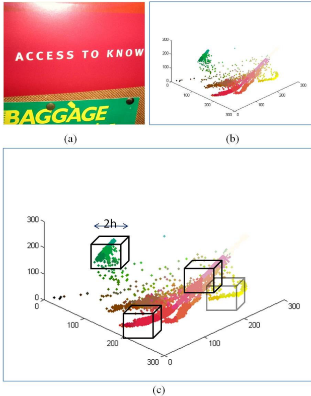
Fig. 7. (a) A scene image with multiple colors; (b) color distribution in RGB space; (c) four of the initial cube color clusters with radius h .
