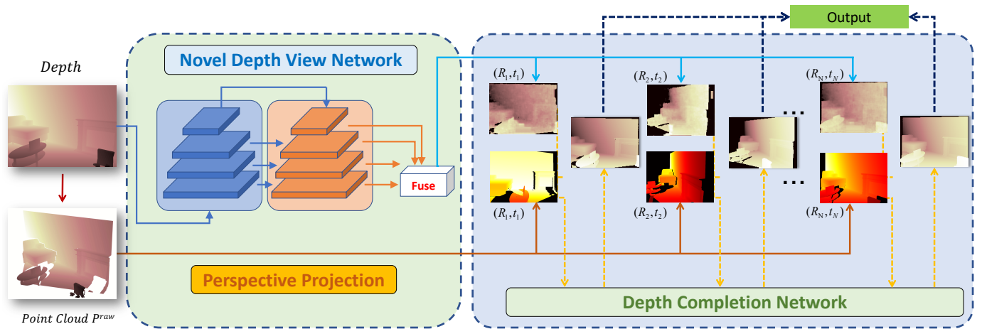
Fig. 2: Architecture of our proposed end-to-end scene point cloud completion network which takes a single depth map with original size as input. The whole structure has two subnetworks: NDVNet (Novel Depth View Network) and DCNet (Depth Completion Network). The NDVNet consists of skip-connected encoder and decoder networks. The pyramid fused feature map outputs are further utilized to predict novel depth maps from various viewpoints ((R_1, t_1), (R_1, t_1) \dots (R_N, t_N)) . Meanwhile, we re-project the point cloud (from input view) to N viewpoints to obtain the coarse depth maps, which can provide more detailed textures. A coarse-to-fine DCNet is then introduced to optimize each viewpoint depth prediction given a novel predicted depth map and a related re-projected coarse depth map. Finally all of the refined depth maps are fused together to form the final completed scene output.
