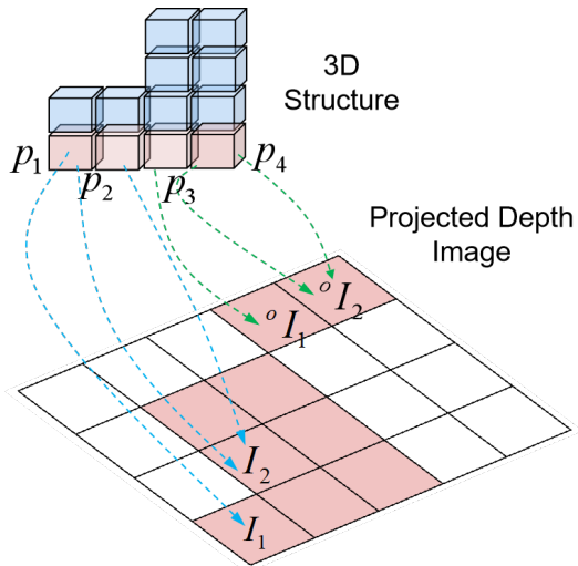
Fig. 3: Coarse depth rendering is performed through a ray-tracing and casting approach, Where the point collision is considered as a fusion to obtain the depth map. Since we use a cube to represent a point in 3D space, there may exist several cubes cast into one pixel or one cube cast into multi-pixels.
