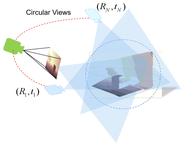
Fig. 4: Illustration of the novel views which are designed in a circular pattern to provide full-coverage of a target scene. The circle is formed by the camera center and the scene center with a fixed height Z .
