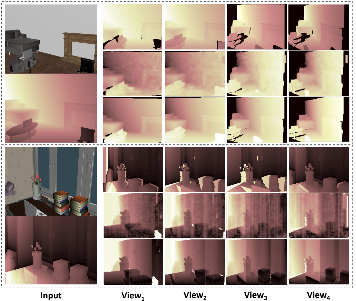
Fig. 6: Qualitative Results of 2 different indoor scenes (divided by the dashed line bounding boxes). For each scene, the first column is the RGB image and input depth map (RGB image is just for visualization and not used in our framework). The other columns are the depth maps of the experiment results under 4 novel views. The first row is the re-projected depth maps under the v_i , which have holes such as desks and floor. The second row is the coarse-completed depth maps generated by NDVNet. And the third row is the final completed depth maps generated by DCNet. Note that the holes are filled and the scenes are well completed through our proposed whole completion model and coarse-to-fine strategy.
