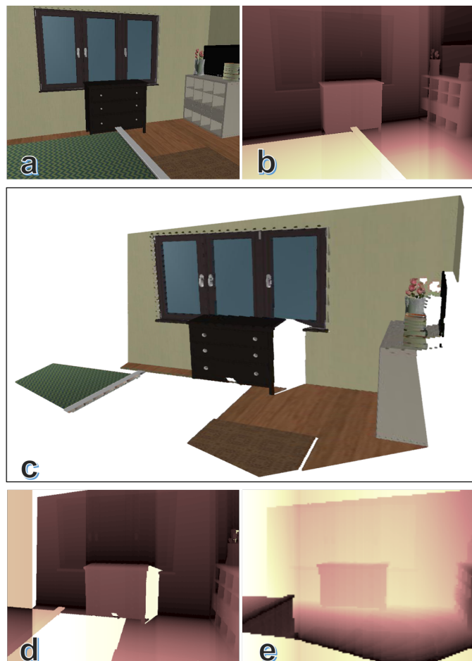
Fig. 1: Illustration of our scene completion via novel depth views: (a) RGB image (for visualization only, and not used in our framework); (b) input depth map; (c) back-projected point cloud visualized from another viewpoint, which shows holes under completion; (d) the incomplete depth map; (e) and the completed depth map with our proposed network. Other views are similar to this view whose holes are filled and thus the scene is completed.
